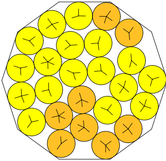
N = 25 25 circles in a decagon
