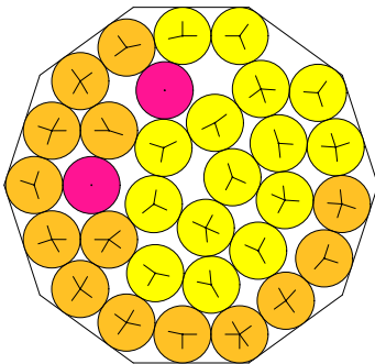
N = 31 31 circles in a decagon
