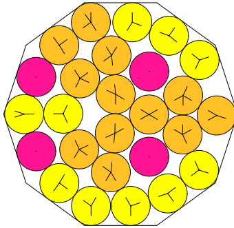
N = 26 26 circles in a decagon
