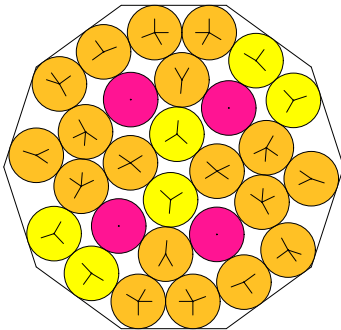
N = 28 28 circles in a decagon
