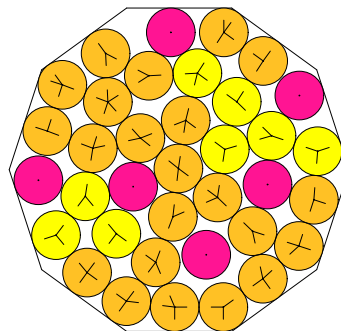
N = 36 36 circles in a decagon
