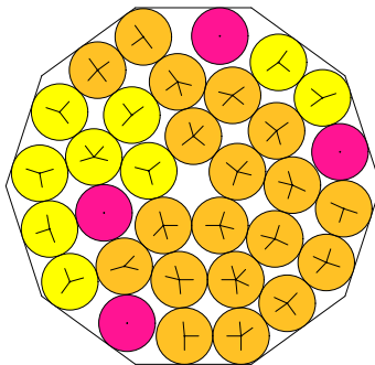
N = 32 32 circles in a decagon
