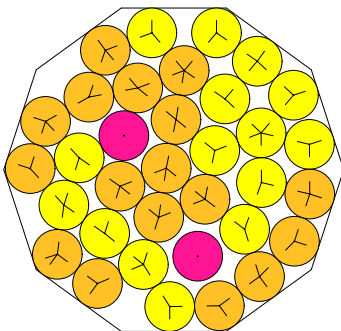
N = 34 34 circles in a decagon
