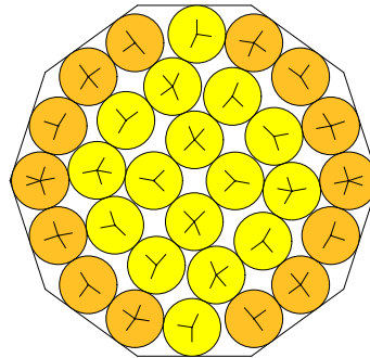
N = 30 30 circles in a decagon
