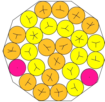
N = 27 27 circles in a decagon
