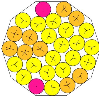
N = 29 29 circles in a decagon
