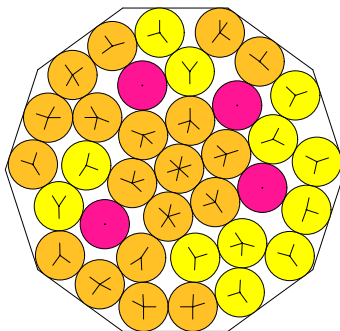
N = 35 35 circles in a decagon
