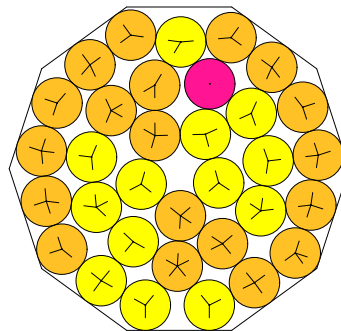
N = 33 33 circles in a decagon
