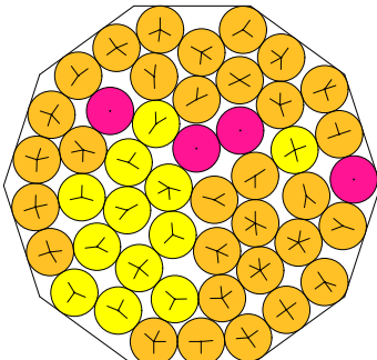
N = 47 47 circles in a decagon
