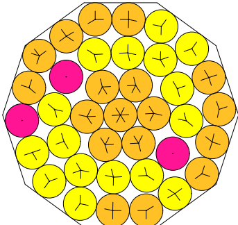
N = 37 37 circles in a decagon
