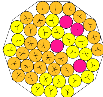
N = 45 45 circles in a decagon
