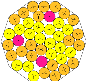
N = 43 43 circles in a decagon
