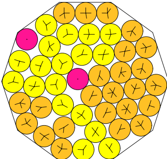
N = 44 44 circles in a decagon
