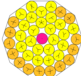
N = 39 39 circles in a decagon
