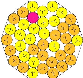
N = 40 40 circles in a decagon
