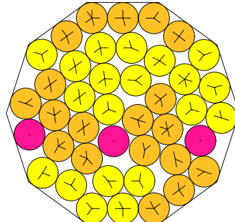
N = 42 42 circles in a decagon
