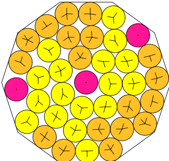
N = 38 38 circles in a decagon
