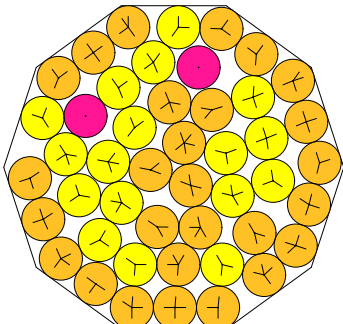
N = 46 46 circles in a decagon
