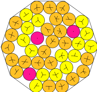
N = 41 41 circles in a decagon
