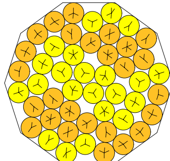
N = 48 48 circles in a decagon
