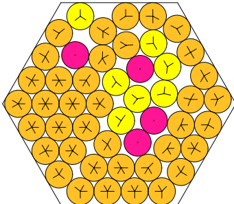
N = 49 49 circles in a hexagon
