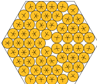
N = 56 56 circles in a hexagon
