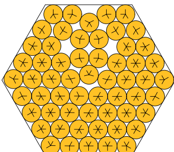
N = 58 58 circles in a hexagon
