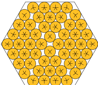
N = 52 52 circles in a hexagon
