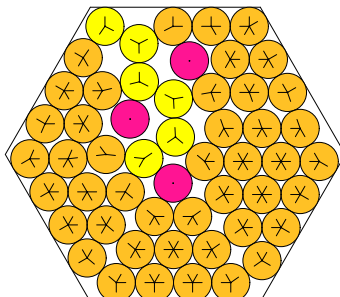
N = 53 53 circles in a hexagon
