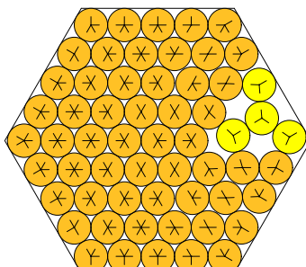
N = 59 59 circles in a hexagon
