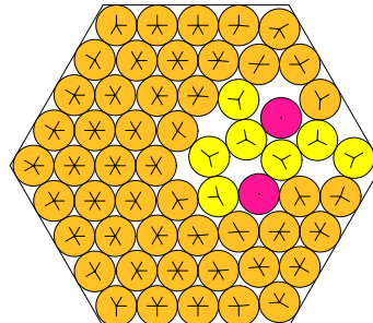
N = 57 57 circles in a hexagon
