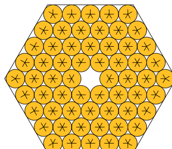
N = 60 60 circles in a hexagon
