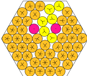
N = 50 50 circles in a hexagon
