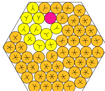
N = 54 54 circles in a hexagon
