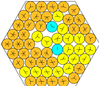
N = 55 55 circles in a hexagon
