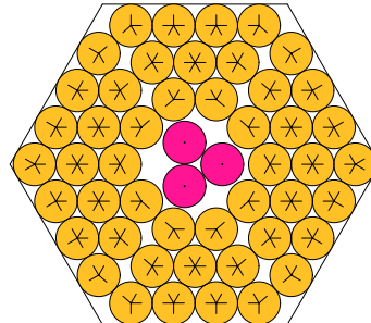
N = 51 51 circles in a hexagon
