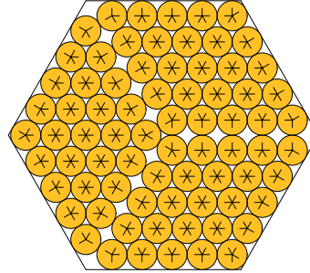
N = 75 75 circles in a hexagon
