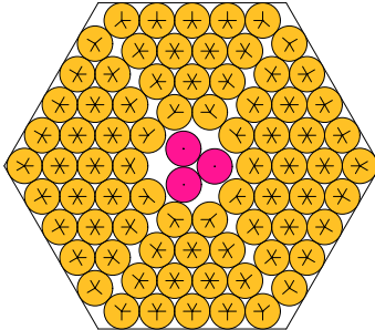
N = 79 79 circles in a hexagon
