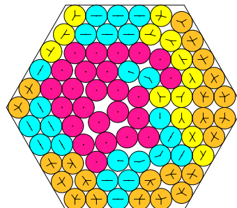
N = 84 84 circles in a hexagon
