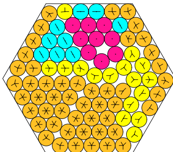
N = 83 83 circles in a hexagon
