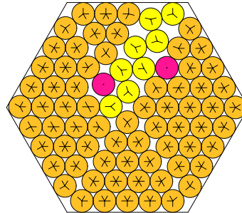
N = 78 78 circles in a hexagon
