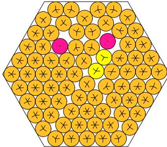
N = 77 77 circles in a hexagon
