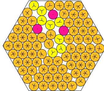
N = 81 81 circles in a hexagon
