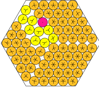
N = 73 73 circles in a hexagon
