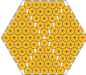
N = 80 80 circles in a hexagon
