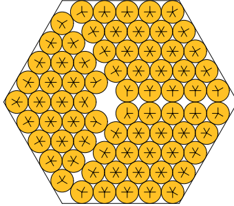
N = 74 74 circles in a hexagon
