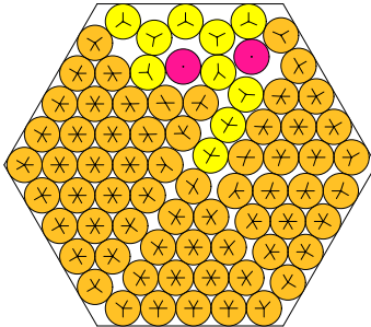
N = 76 76 circles in a hexagon
