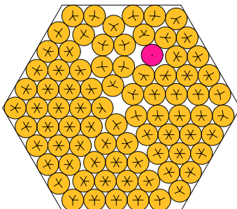
N = 82 82 circles in a hexagon
