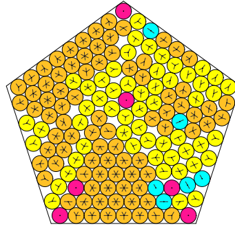
N = 150 150 circles in a pentagon
