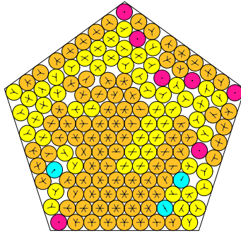
N = 152 152 circles in a pentagon
