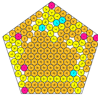
N = 156 156 circles in a pentagon
