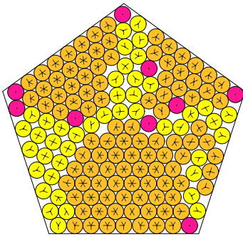
N = 154 154 circles in a pentagon
