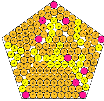
N = 149 149 circles in a pentagon
