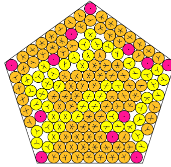
N = 147 147 circles in a pentagon
