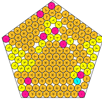
N = 146 146 circles in a pentagon
