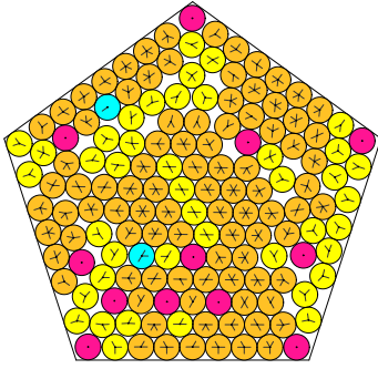
N = 148 148 circles in a pentagon
