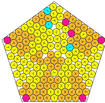
N = 155 155 circles in a pentagon
