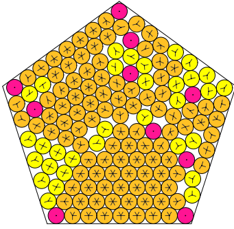
N = 145 145 circles in a pentagon
