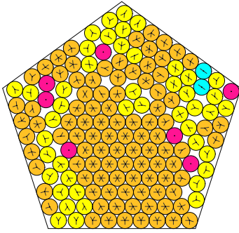
N = 151 151 circles in a pentagon
