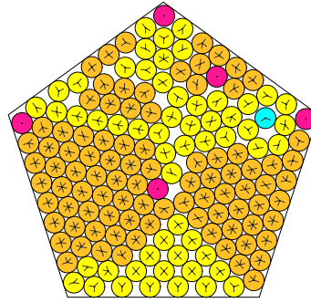
N = 153 153 circles in a pentagon
