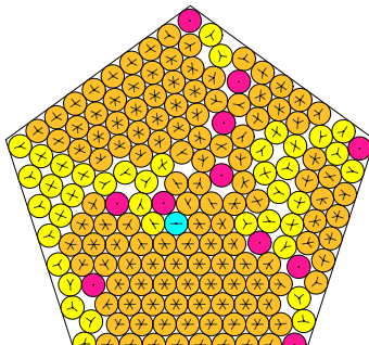
N = 176 176 circles in a pentagon
