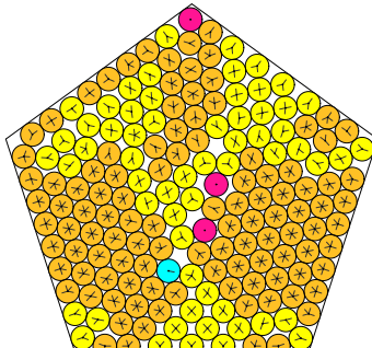
N = 173 173 circles in a pentagon
