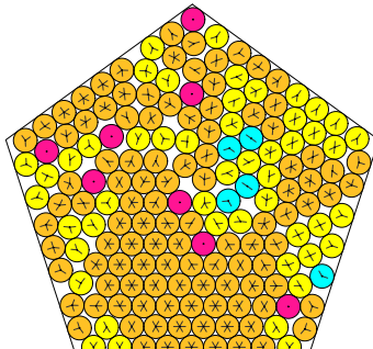
N = 170 170 circles in a pentagon
