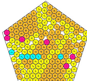
N = 171 171 circles in a pentagon
