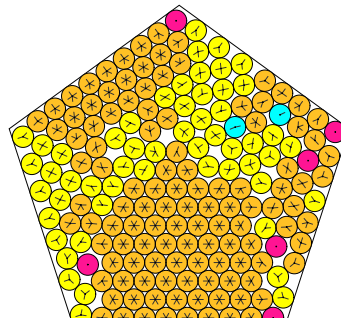
N = 177 177 circles in a pentagon
