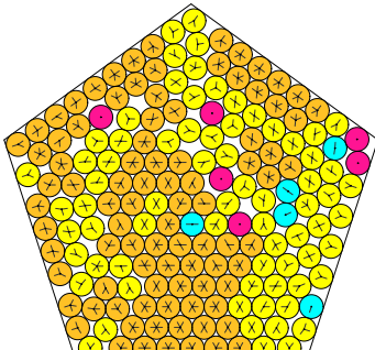
N = 172 172 circles in a pentagon
