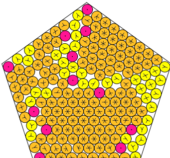
N = 178 178 circles in a pentagon
