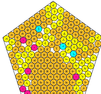
N = 174 174 circles in a pentagon
