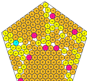
N = 179 179 circles in a pentagon
