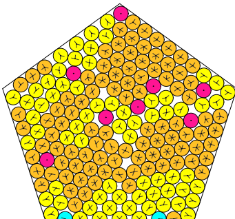
N = 175 175 circles in a pentagon
