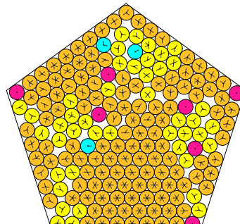
N = 180 180 circles in a pentagon
