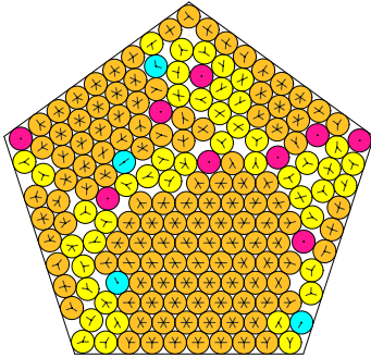
N = 181 181 circles in a pentagon
