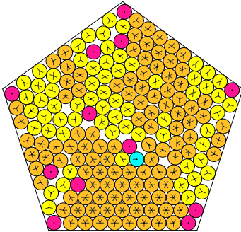
N = 187 187 circles in a pentagon
