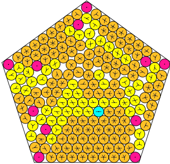
N = 184 184 circles in a pentagon
