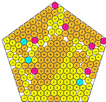
N = 191 191 circles in a pentagon
