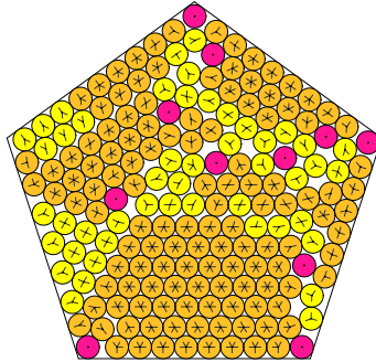
N = 185 185 circles in a pentagon
