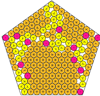
N = 182 182 circles in a pentagon
