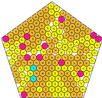
N = 190 190 circles in a pentagon
