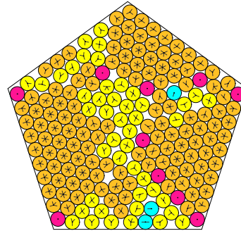
N = 189 189 circles in a pentagon
