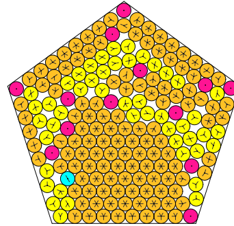
N = 183 183 circles in a pentagon
