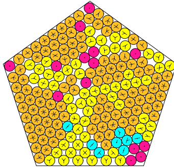
N = 188 188 circles in a pentagon
