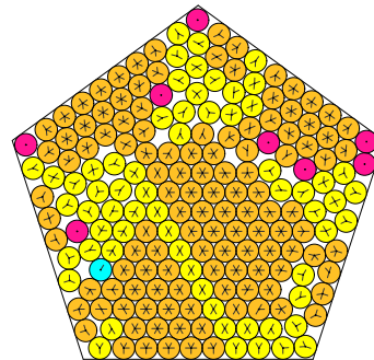
N = 192 192 circles in a pentagon
