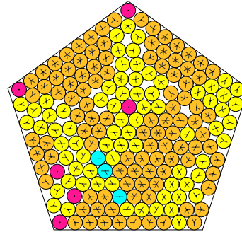
N = 186 186 circles in a pentagon
