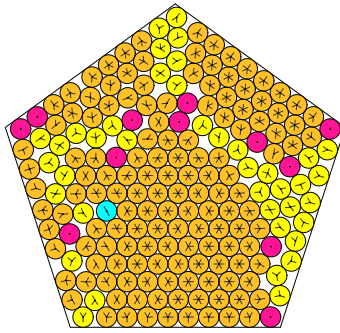
N = 194 194 circles in a pentagon
