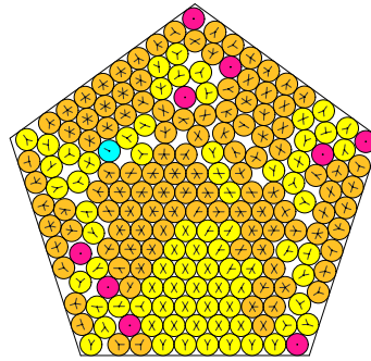
N = 198 198 circles in a pentagon
