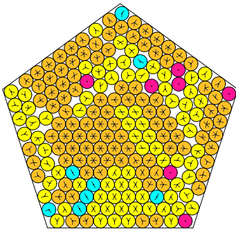
N = 199 199 circles in a pentagon
