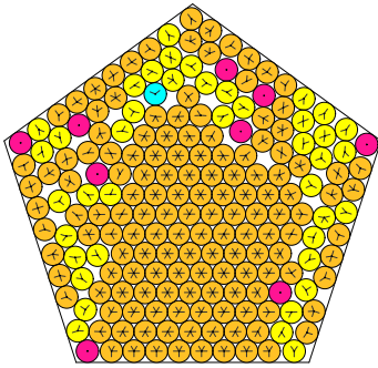
N = 196 196 circles in a pentagon
