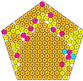
N = 197 197 circles in a pentagon
