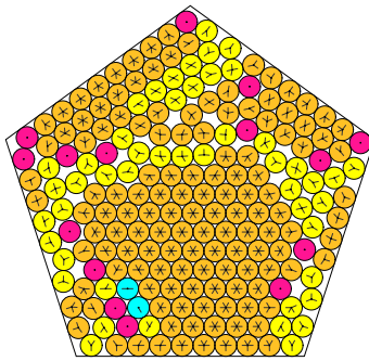
N = 200 200 circles in a pentagon
