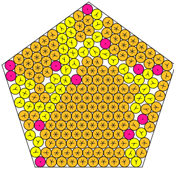
N = 193 193 circles in a pentagon
