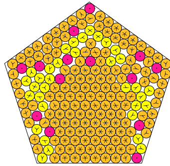
N = 195 195 circles in a pentagon
