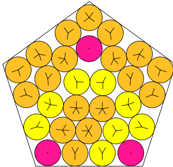
N = 29 29 circles in a pentagon
