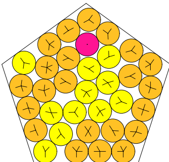
N = 34 34 circles in a pentagon
