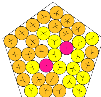
N = 36 36 circles in a pentagon
