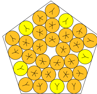
N = 30 30 circles in a pentagon
