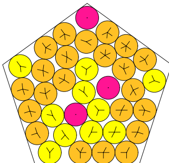
N = 35 35 circles in a pentagon
