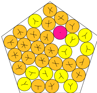
N = 32 32 circles in a pentagon
