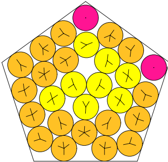
N = 28 28 circles in a pentagon
