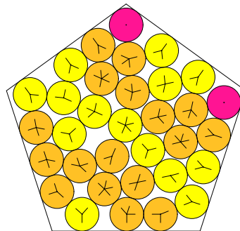
N = 33 33 circles in a pentagon
