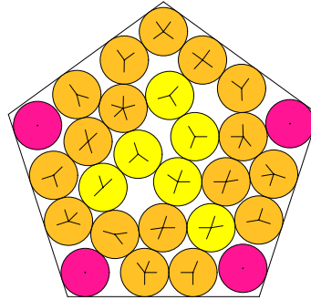
N = 27 27 circles in a pentagon
