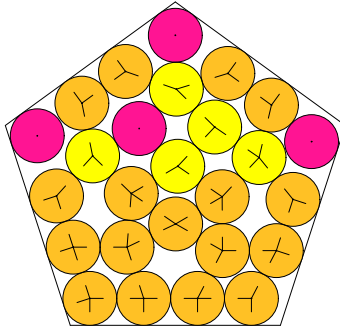
N = 26 26 circles in a pentagon
