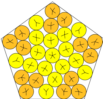
N = 31 31 circles in a pentagon
