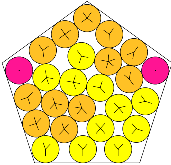
N = 25 25 circles in a pentagon
