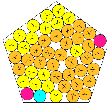
N = 48 48 circles in a pentagon
