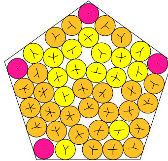
N = 45 45 circles in a pentagon
