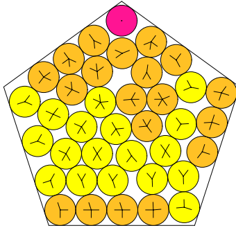
N = 38 38 circles in a pentagon
