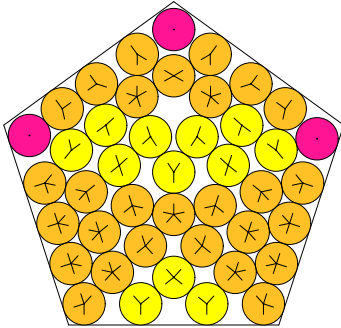
N = 43 43 circles in a pentagon
