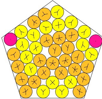
N = 41 41 circles in a pentagon
