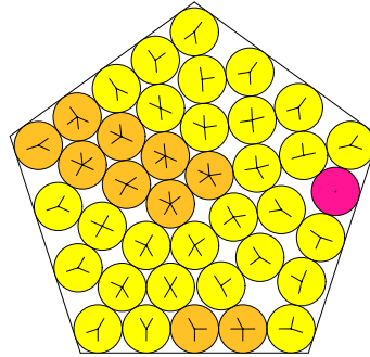
N = 39 39 circles in a pentagon
