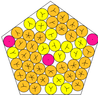
N = 47 47 circles in a pentagon
