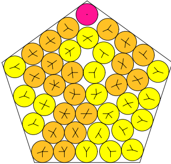
N = 40 40 circles in a pentagon
