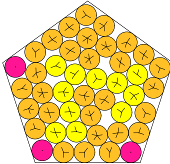
N = 44 44 circles in a pentagon
