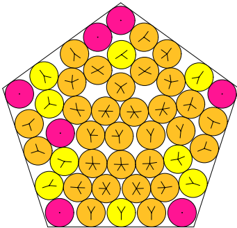
N = 46 46 circles in a pentagon
