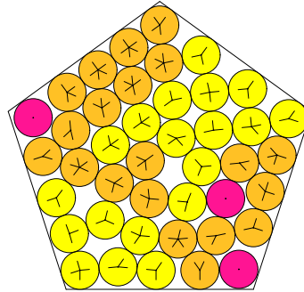
N = 42 42 circles in a pentagon
