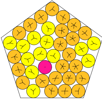
N = 37 37 circles in a pentagon
