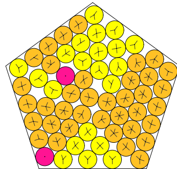
N = 60 60 circles in a pentagon
