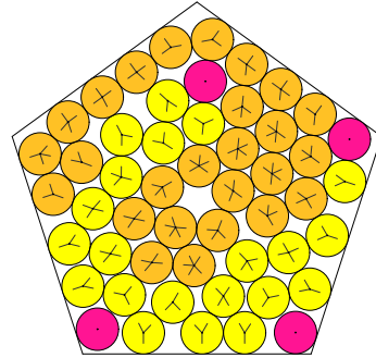
N = 51 51 circles in a pentagon
