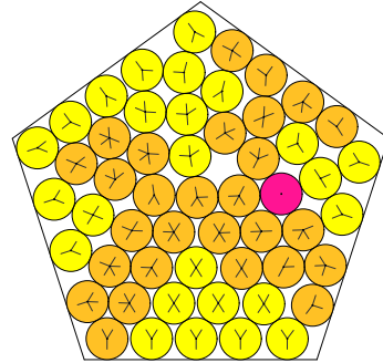
N = 54 54 circles in a pentagon
