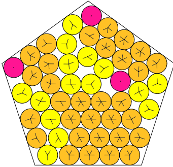
N = 49 49 circles in a pentagon
