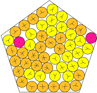
N = 52 52 circles in a pentagon
