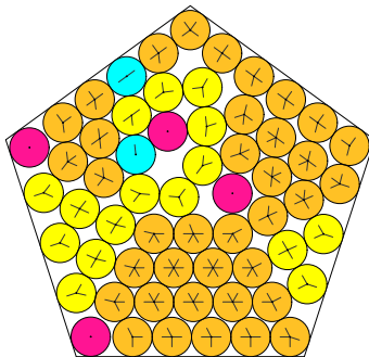
N = 59 59 circles in a pentagon
